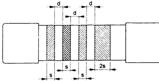
Figure A.1 – Layout of colour bands
